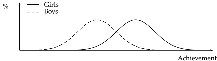
Figure 1: SHIFT
